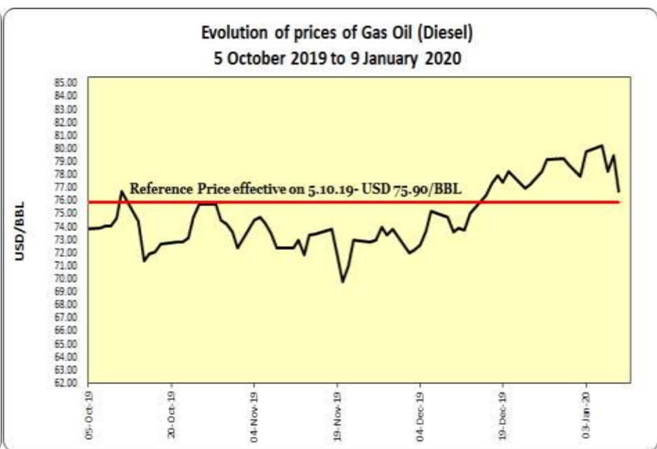
Graph 2 – Gas Oil
